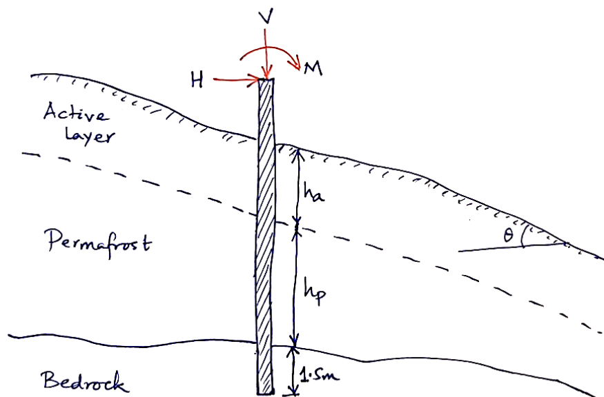
Figure 7: Representative model for pile response analysis.
